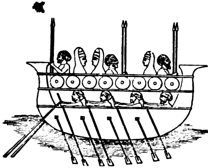
Galley. (Xouyunjik.)
